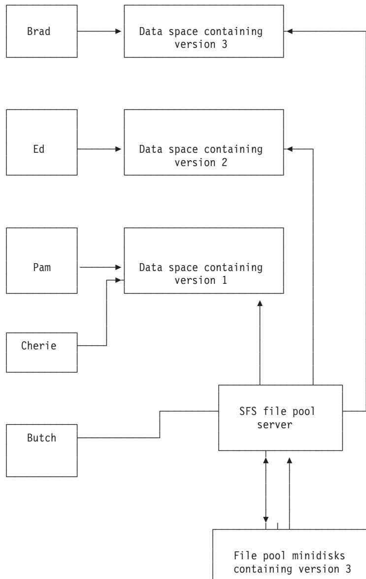
Figure 35. Using Directory Control Directories
